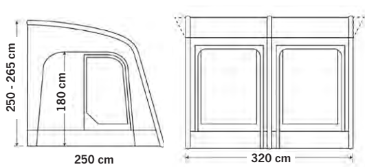
Optionally ventilated ceiling
