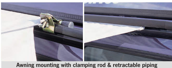
Awning mounting with clamping rod & retractable piping
