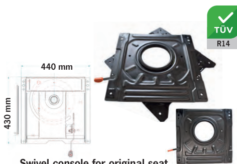
Swivel console for original seat
