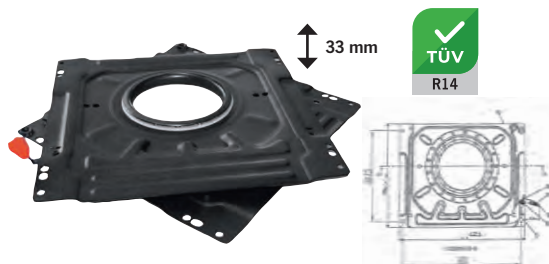
Swivel console for original seat
