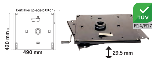
Swivel console for original seat
