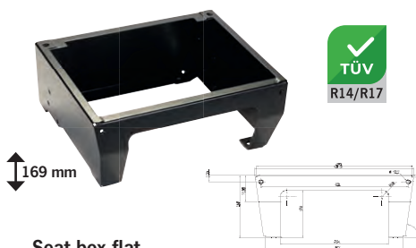
Seat box flat Instead of original box.
