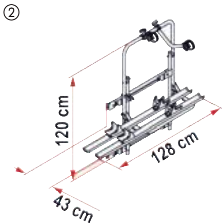
Carry-Bike 200 DJ
