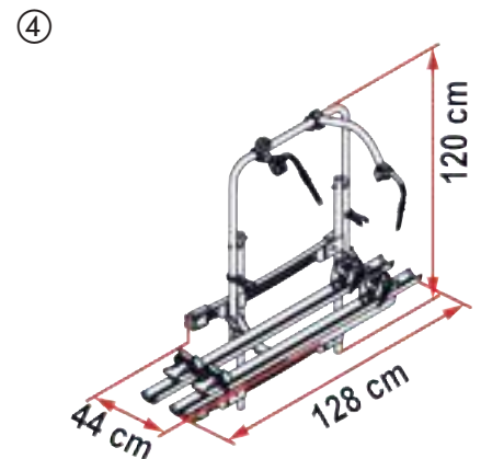
Carry-Bike 200 DJ
